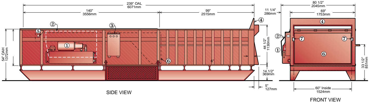
Concrete Pad Requirements 6" (153mm) Thick Reinforced 3000 PSI Concrete, 10'-0"W x 45'-0"L (3.05m x 13.7m), (8) 3/4" (20mm) Anchor Bolts (Min.)
